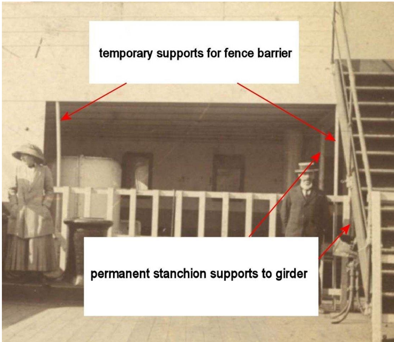
Permanent stanchion supports to poop deck girder
