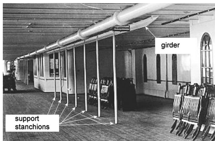
Support stanchions to boat deck girder
